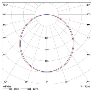
AXOR 53 LED 4400lm 840 opal
